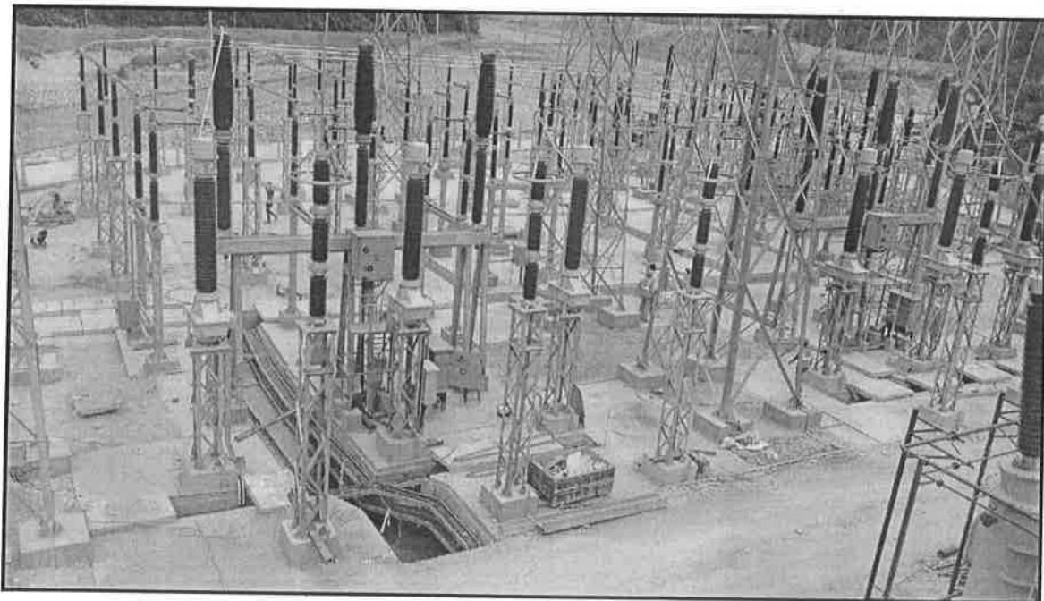
Switchyard
